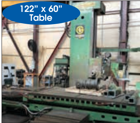
6" GIDDINGS & LEWIS G60T CNC TABLE TYPE HORIZONTAL BORING MILL
