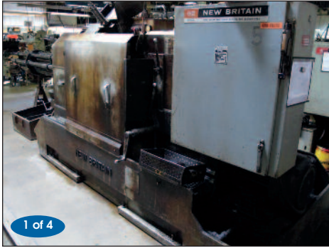
NEW BRITAIN #62 MULTI-SPINDLE SCREW MACHINE
