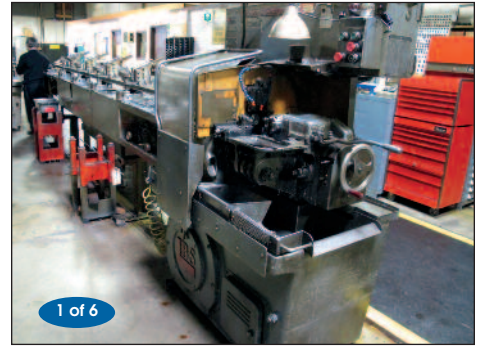
B&S #2 AUTOMATIC SCREW MACHINE
