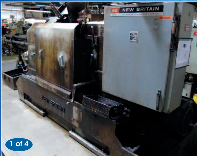
NEW BRITAIN #62 MULTI-SPINDLE SCREW MACHINE
