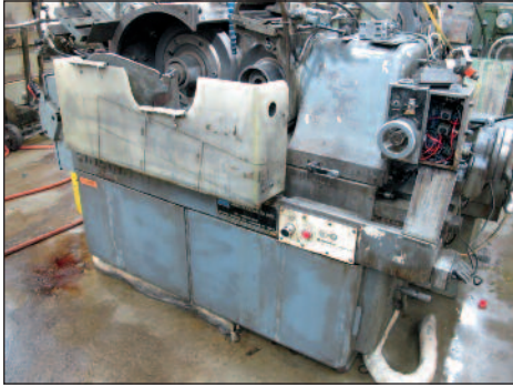
CINCINNATI CENTERLESS GRINDER
