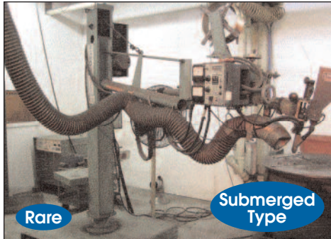
PANDJIRIS # 172 WELDING MANIPULATOR
