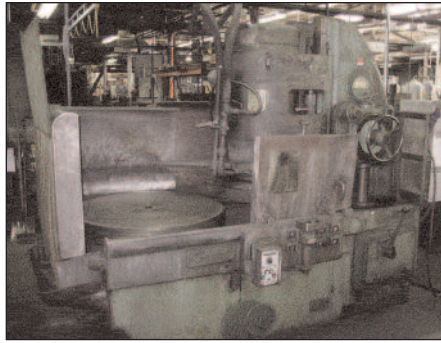
BLANCHARD # 18-36" ROTARY SURFACE GRINDER
