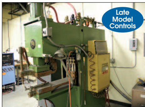
Banner Rocker Arm Spot Welder Model RAP150-24
