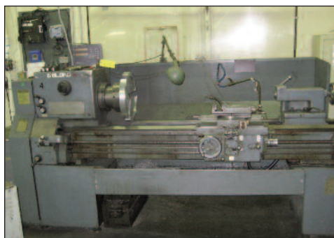
Leblond 24" x 60" Engine lathe
