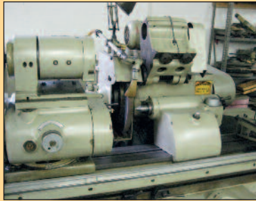
SMTW # MQ14-320 X 1500 "UNIVERSAL" CYLINDRICAL GRINDER
