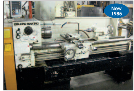
LEBLOND-MAKINO # REGAL "SERVO SHIFT" ENGINE LATHE
