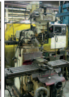
ACER 3 HP VERTICAL MILLING MACHINE W/Proto-Trak MX-2 CNC Control
