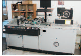
Kirk Rudy NetJet Variable Data Print System
