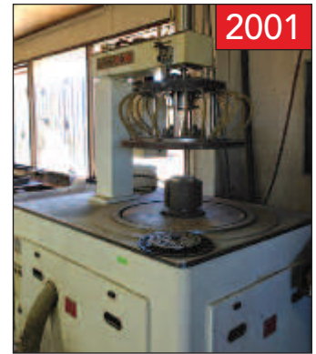
SPEEDFAM AUTO. VERT. LAPPING MACHINE
