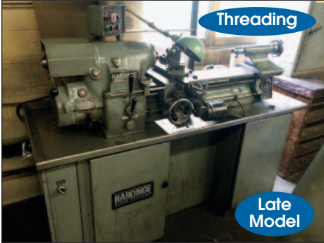
Hardinge Super Precision Toolroom Lathe # HLH
