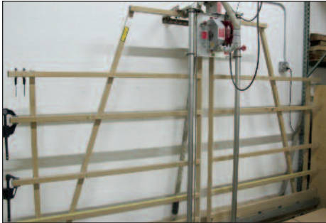
Safety Speed Cut Panel Saw Model H5
